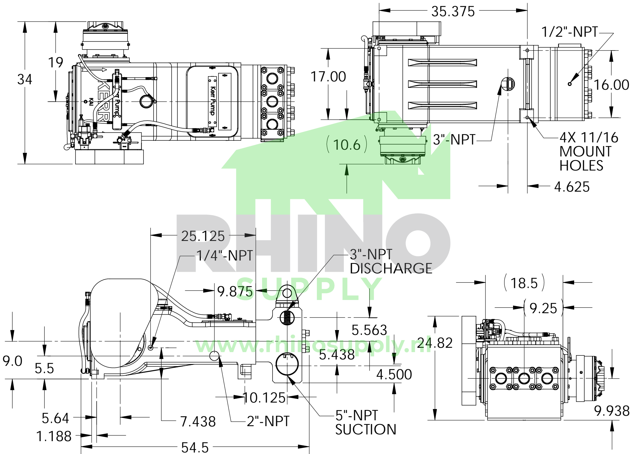
GENERAL DIMENSIONS FOR KA-3500PT
