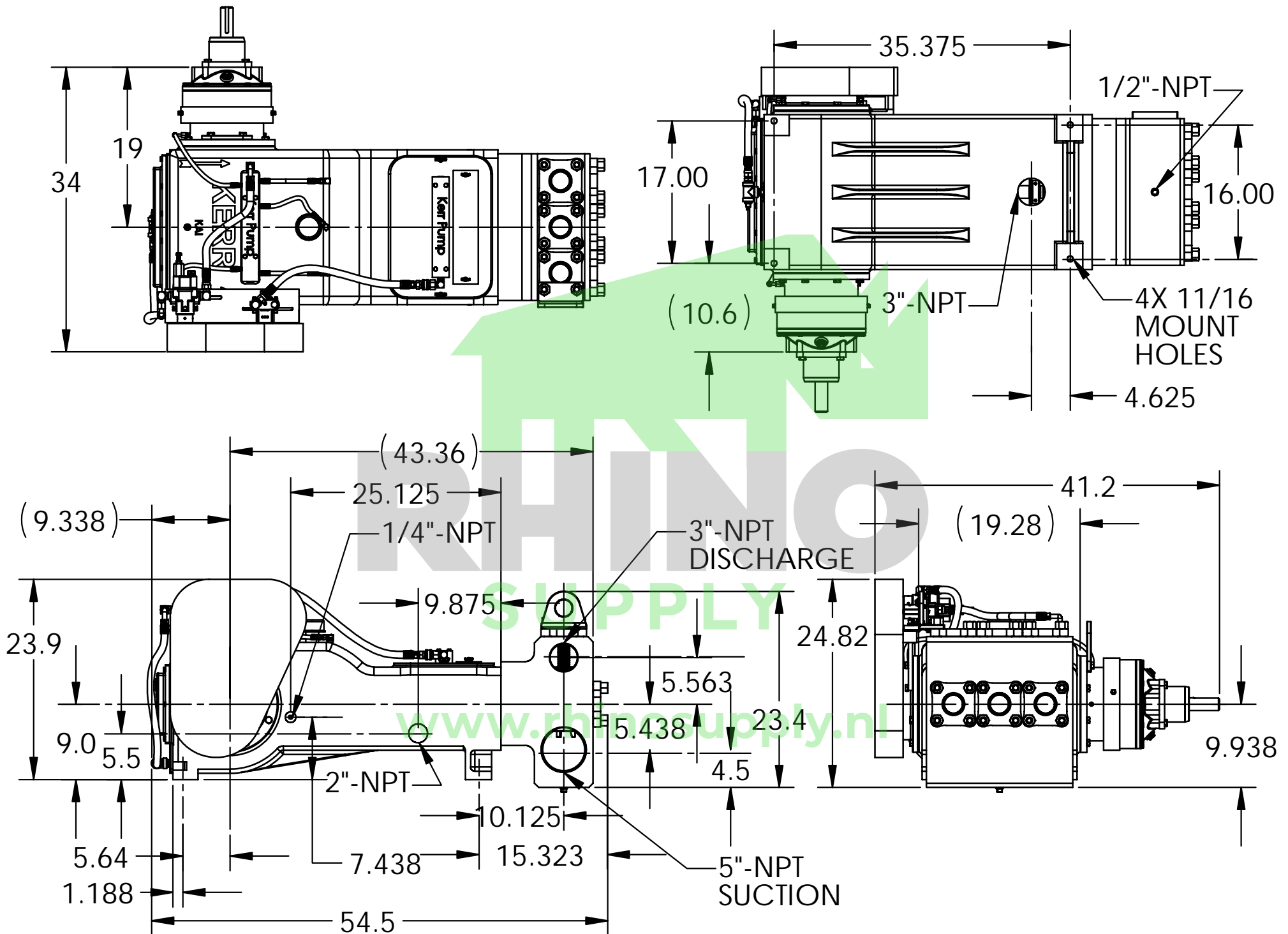
GENERAL DIMENSIONS FOR KA-3500PT WITH DRIVE ASSEMBLY
