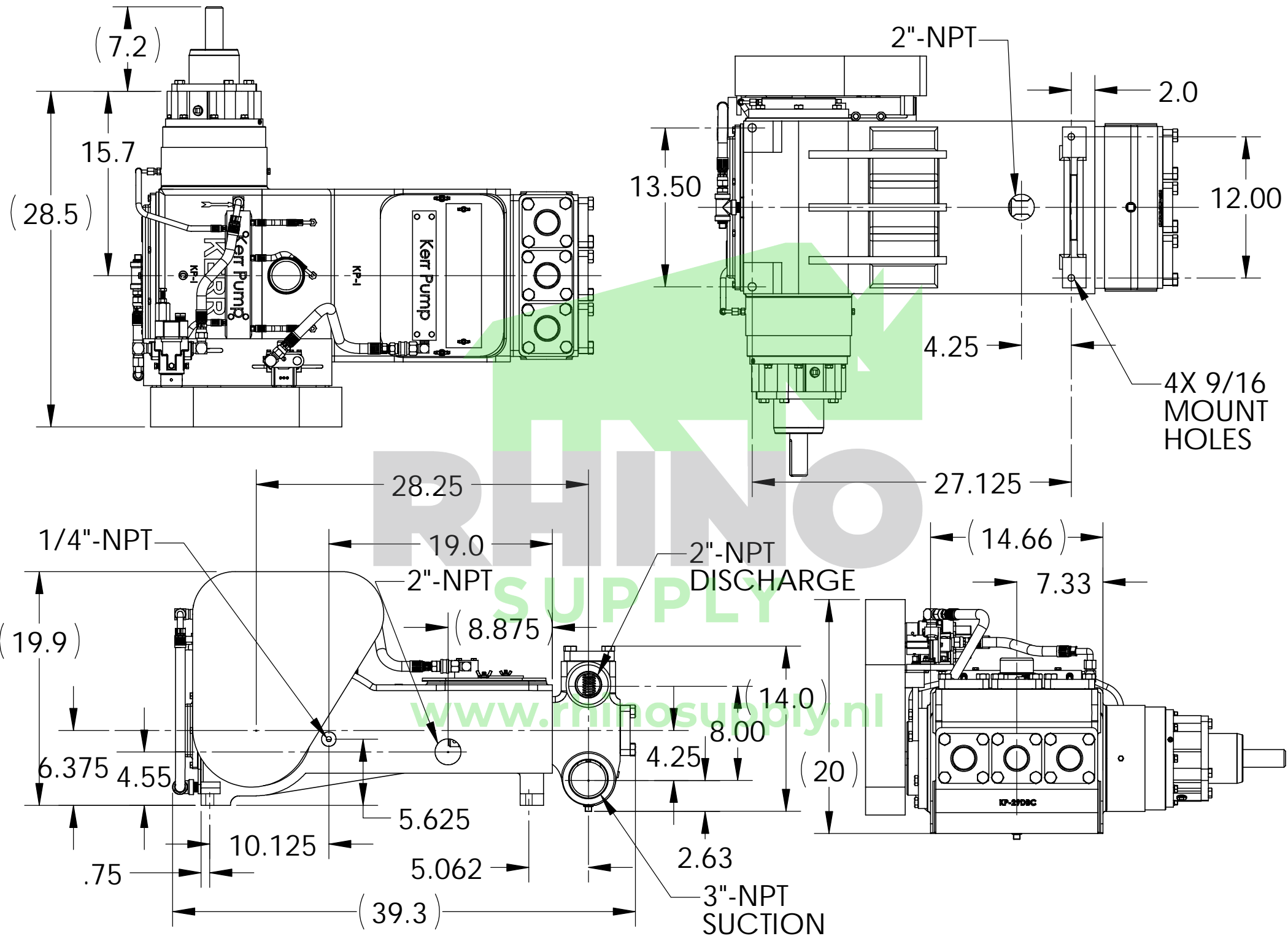
GENERAL DIMENSIONS FOR KP-3300PTHD
